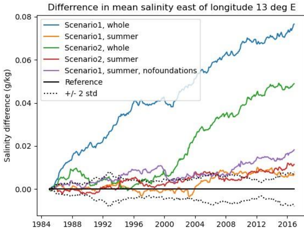
Figure 3: Change in mean salinity east of longitude 13°E for all runs. The change is relative to the mean of the reference runs. The interval +/- 2 standard deviations of the reference runs are shown with dotted lines.
